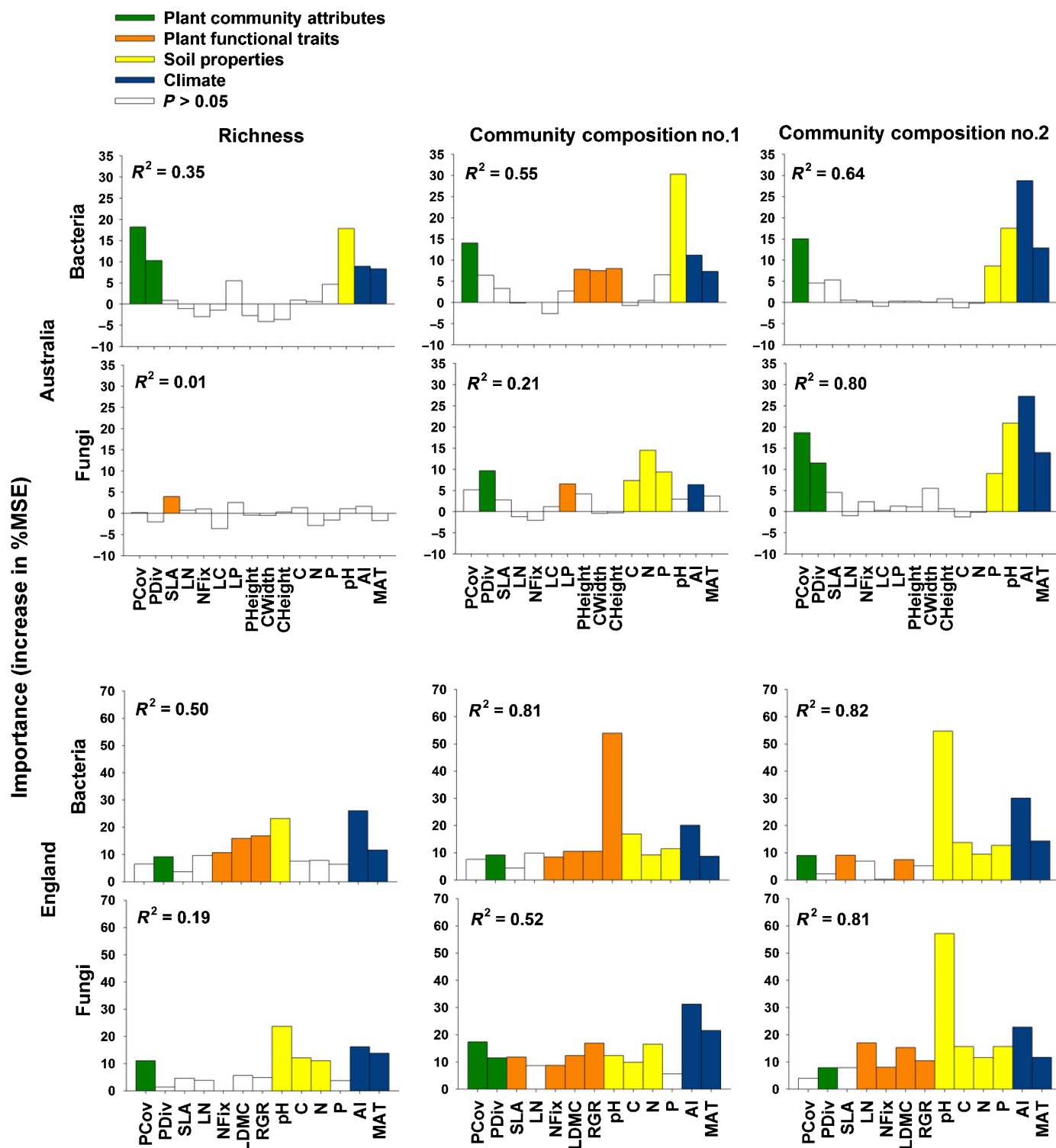
Fig. 3 Random forest analysis aiming to identify the best individual predictors of the diversity and community composition of bacteria and fungi in Australia and England. Predictors include plant attributes, soil properties and climate (Table 1). MSE, mean square error. Community compositions no. 1 and no. 2 represent the first and second axes of a nonmetric multidimensional scaling including the community composition of bacteria or fungi (see Fig. S3).
